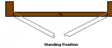
Clockwise Opening Rebated Equal Pair
