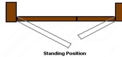
Clockwise Opening Hospital Doorset
